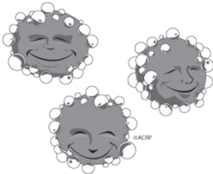
Figure 12.5 - Hydrophilic Particles
