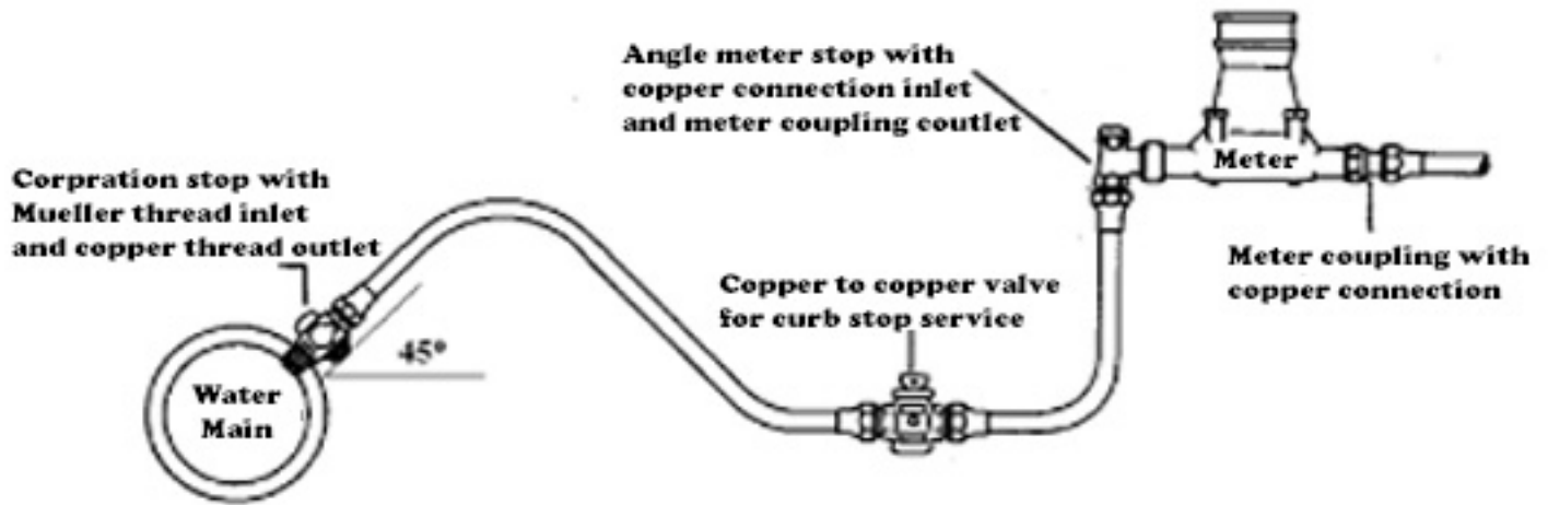
Figure 7.19 - Service Line Installation
