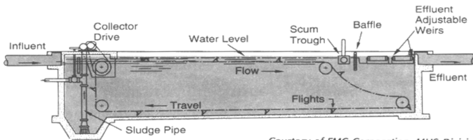
Figure 12.13 - Rectangular Sedimentation Basin
