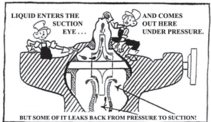
Figure 9.9 - Leak Back
