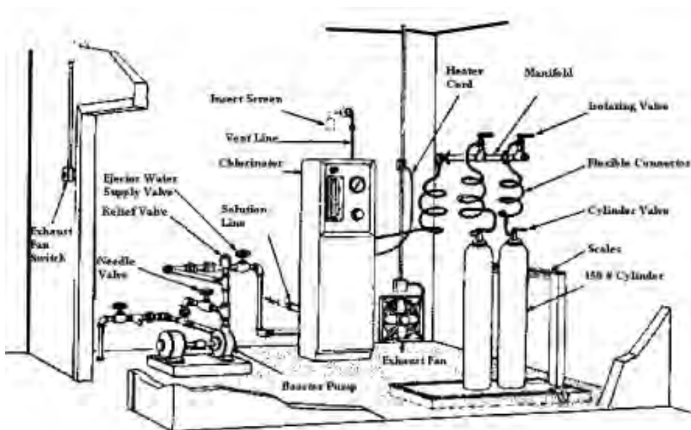
Figure 5.3 - Gas Chlorine Installation (150 Lb. Cylinders)
