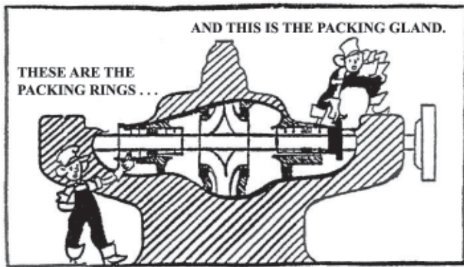
Figure 9.10 - Stuffing Material
