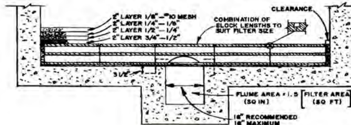
Figure 12.18 - Filter Underdrain System
