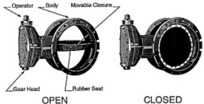
Figure 7.16 - Butterfly Valve
