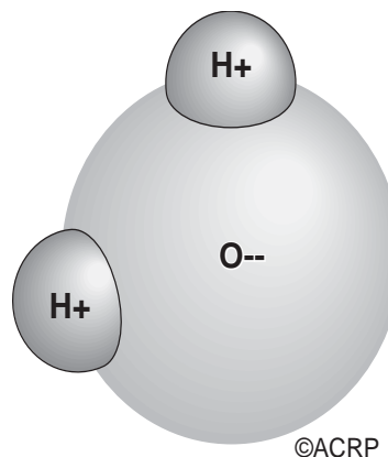
Figure 3.2 - Water Molecule
