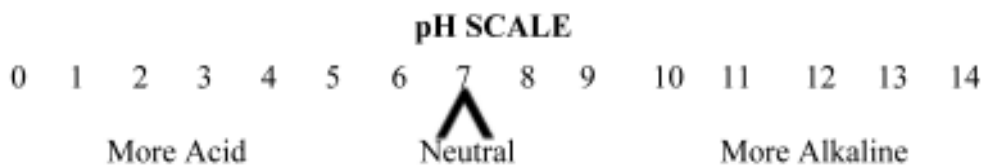
Figure 12.2 - pH Scale
