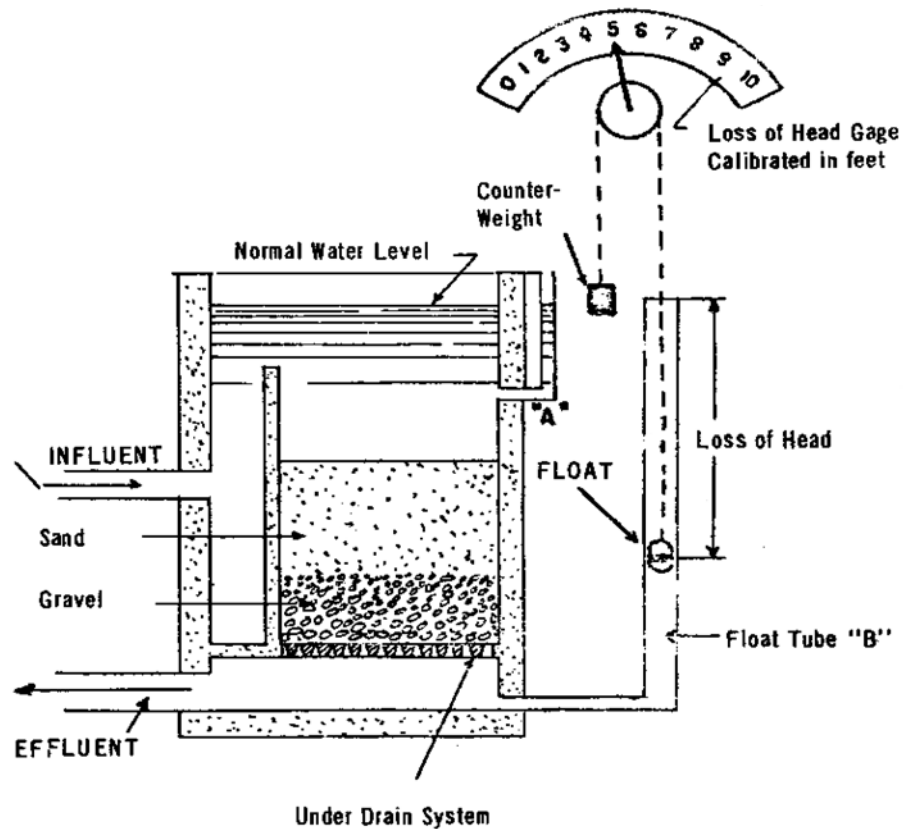
Under Drain System Figure 12.20 - Loss of Head Gauge
