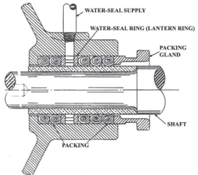
Figure 9.12 - Stuffing Box Cross-Section
