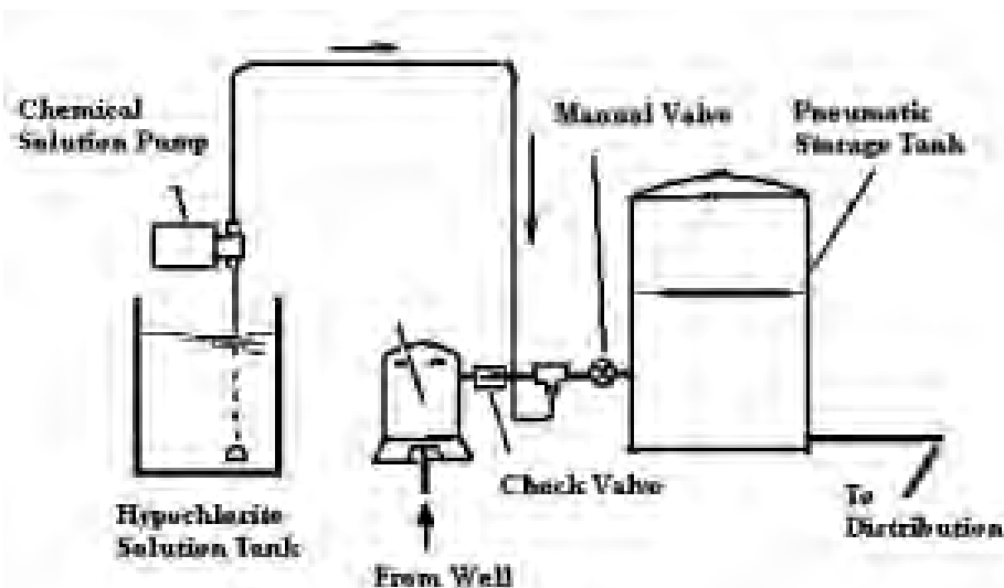
Figure 5.6 - Typical Hypochlorination System
