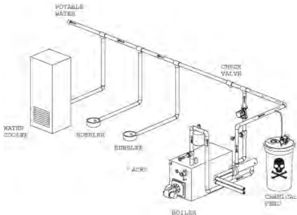
Figure 7.24 - Backpressure with boilers
