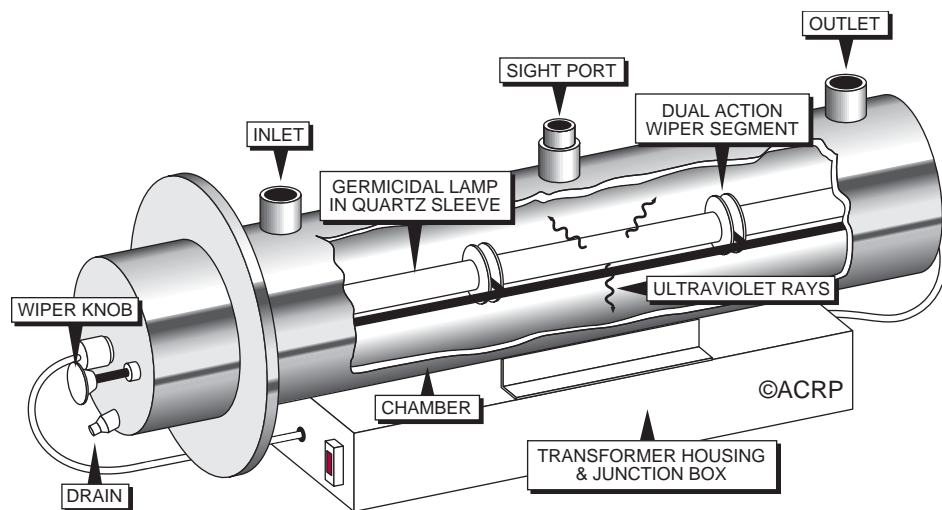
Figure 5.7 - UV Disinfection System
