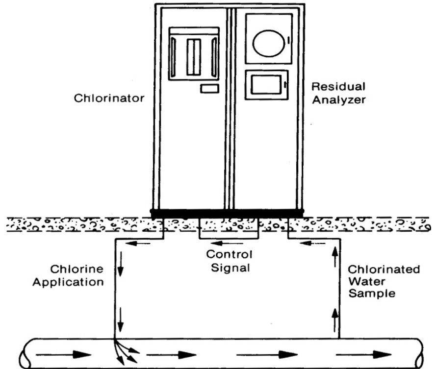
Figure 10.5 - Feedback Control Loop
