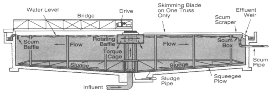
Figure 12.14 - Circular Sedimentation Basin
