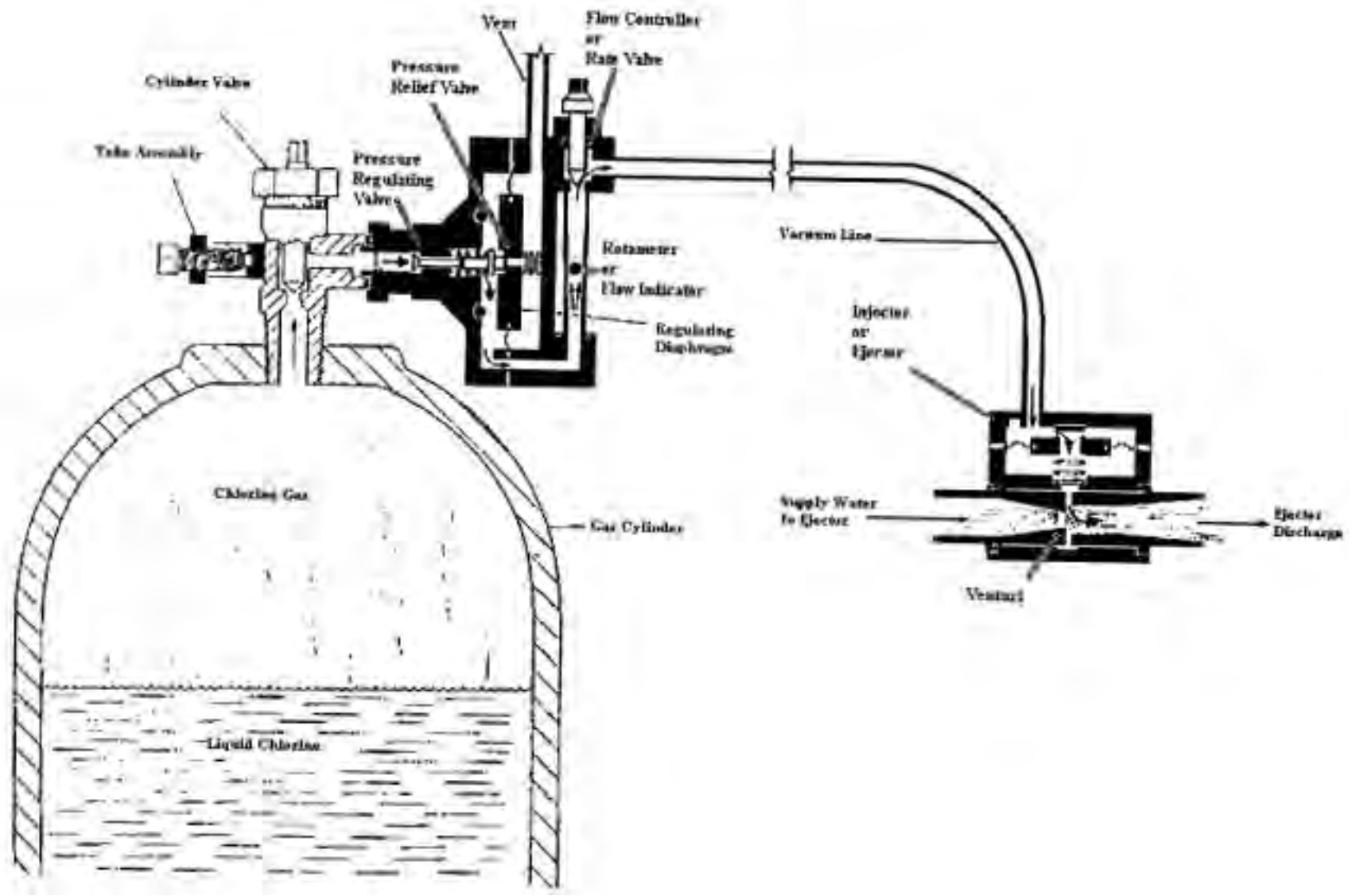
Figure 5.5 - 150 lb Chlorine Gas Feed Unit
