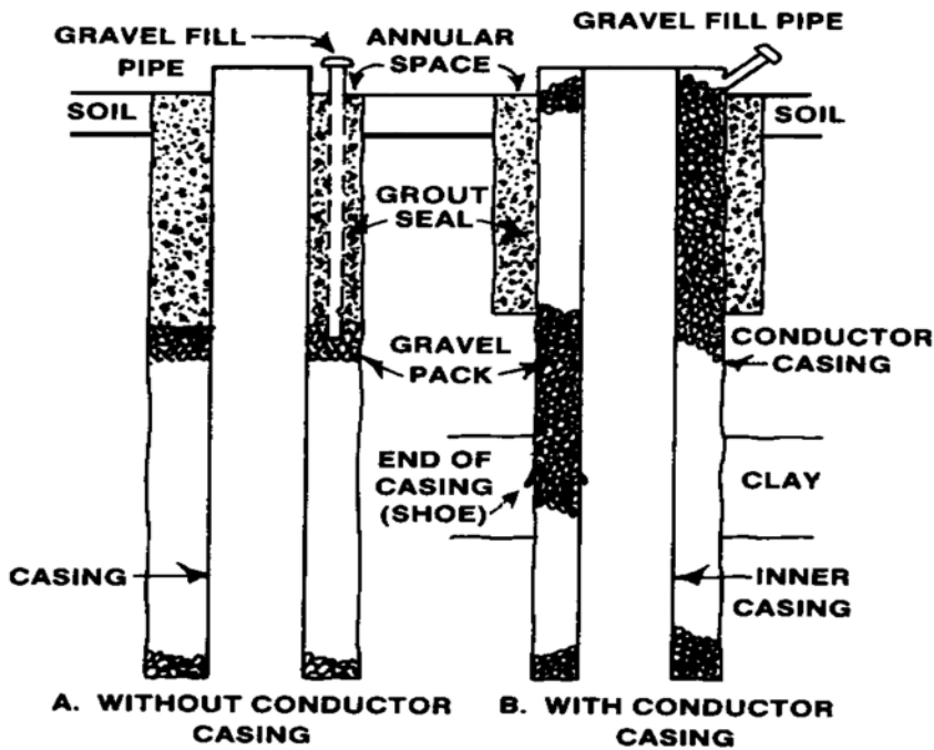
Figure 11.5 - Gravel Packed Well Types
