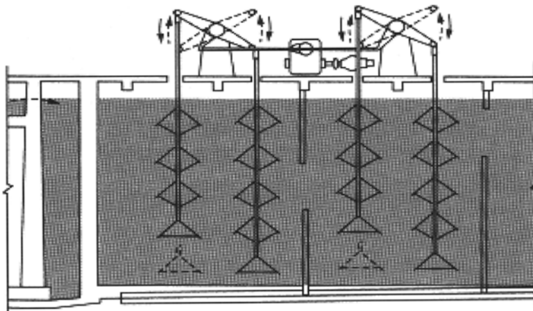
Walking-Beam Flocculator
