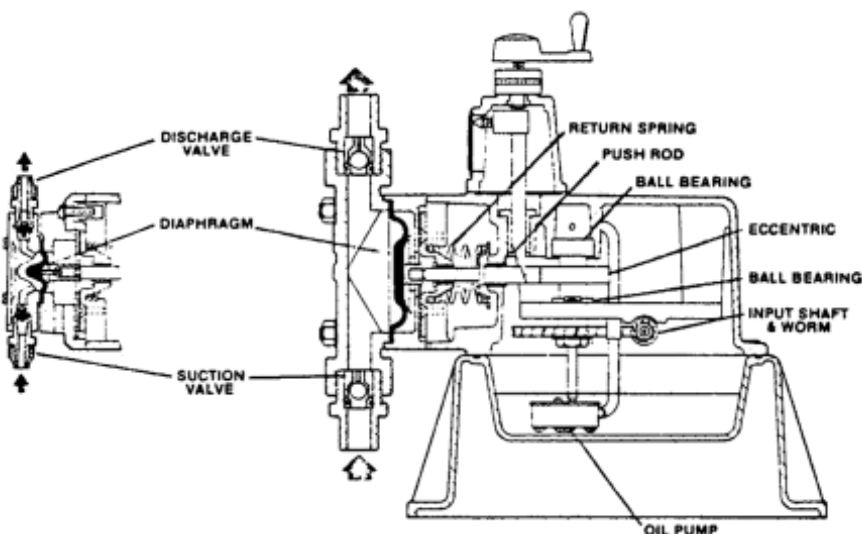
Figure 10.9 - Diaphragm Pump
