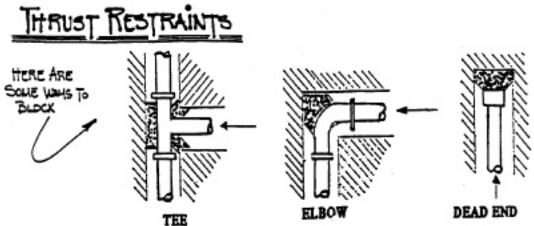
Figure 7.22 - Thrust Restraints
