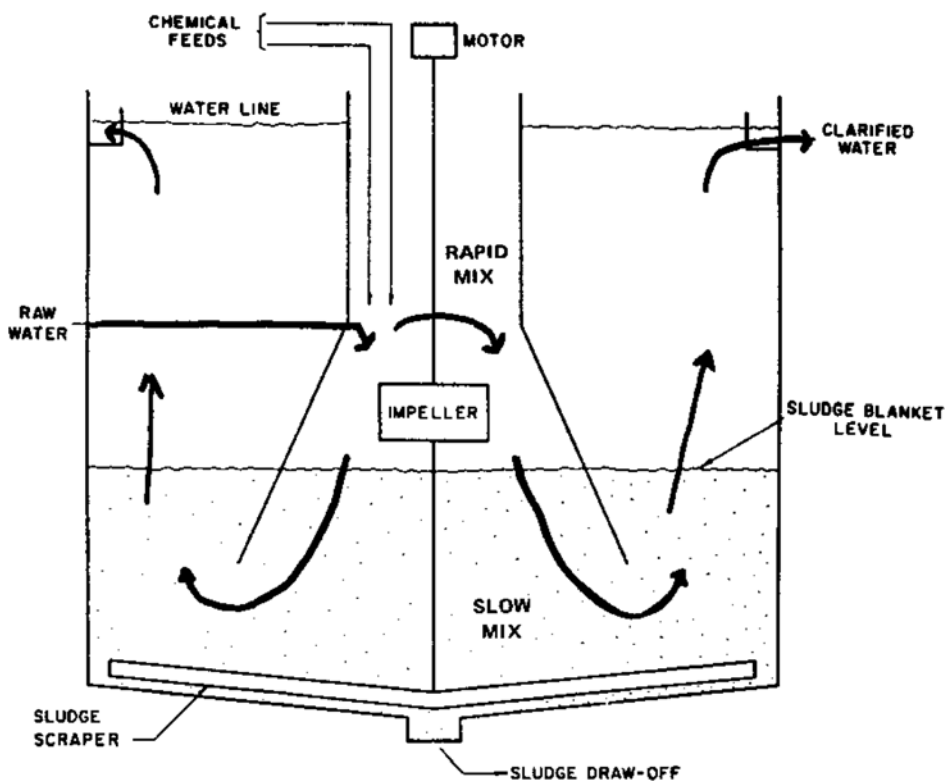
Figure 12.15 - Up-Flow Clarifier
