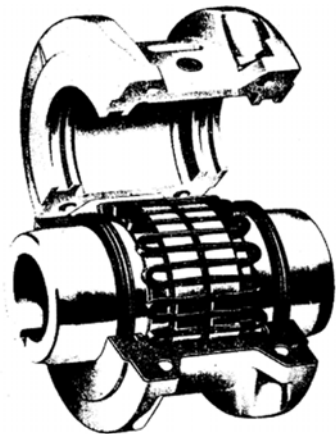
Figure 10.3 - Flexible Grid Coupling
