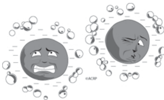
Figure 12.4 - Hydrophobic Particles
