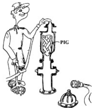
Figure 7.14 - Launching a Pig
