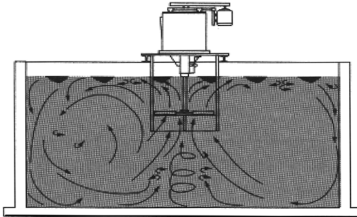
Turbine Flocculator
