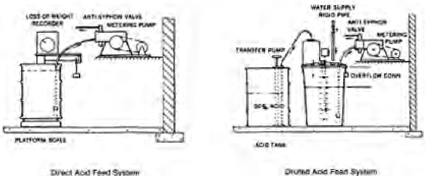
Figure 6.1 - Fluoride Feed Systems
