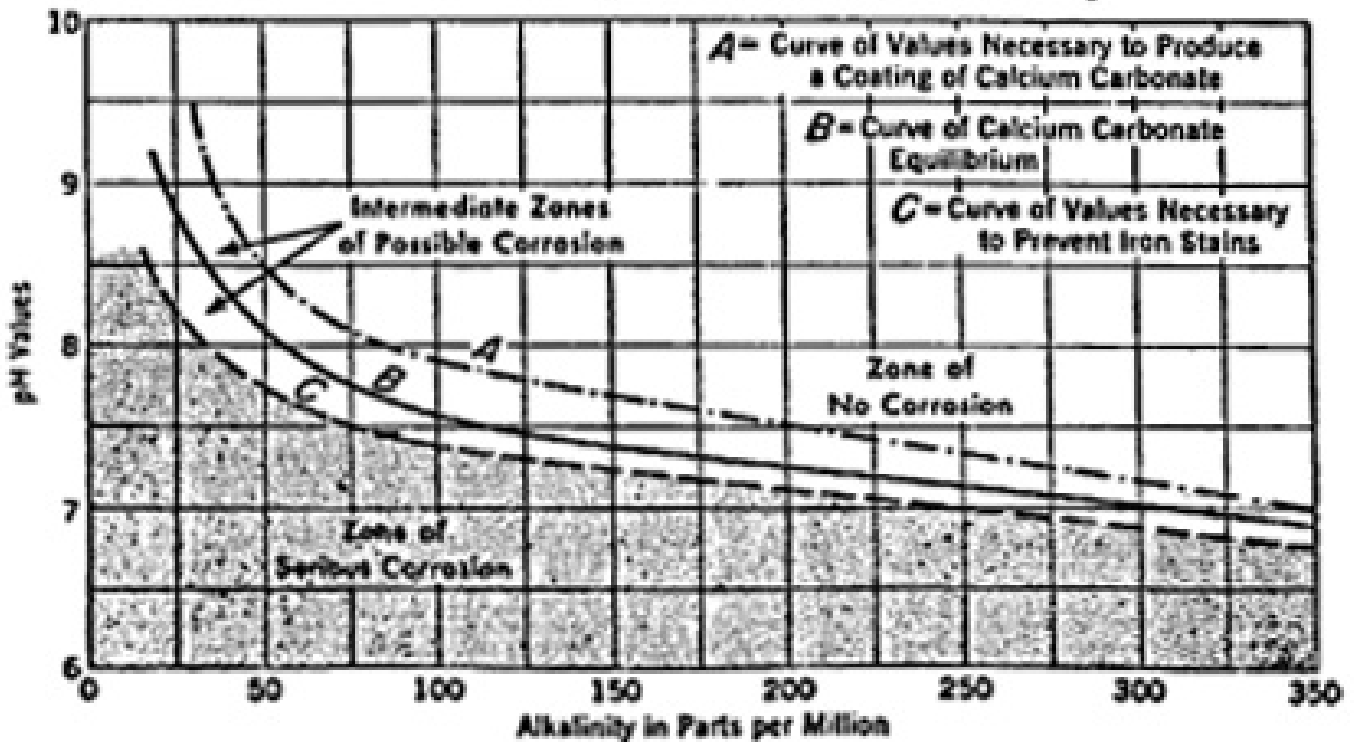
Figure 7.23 - Baylis Curve
