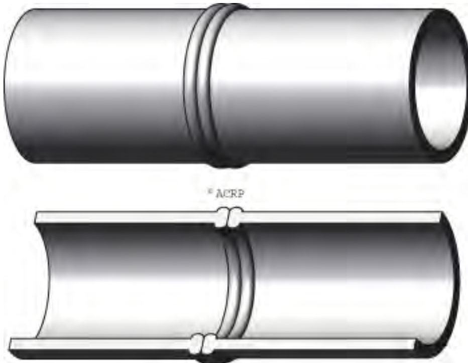
Figure 7.11 - HDPE Heat Fused Welded Joint
