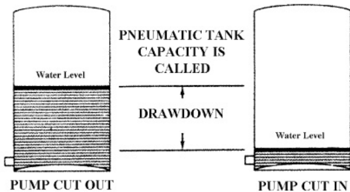
Figure 8.3 - Drawdown
