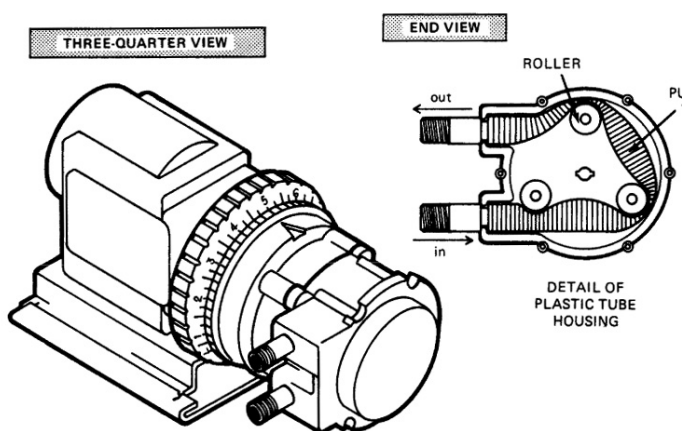
Figure 10.8 - Peristaltic Pump
