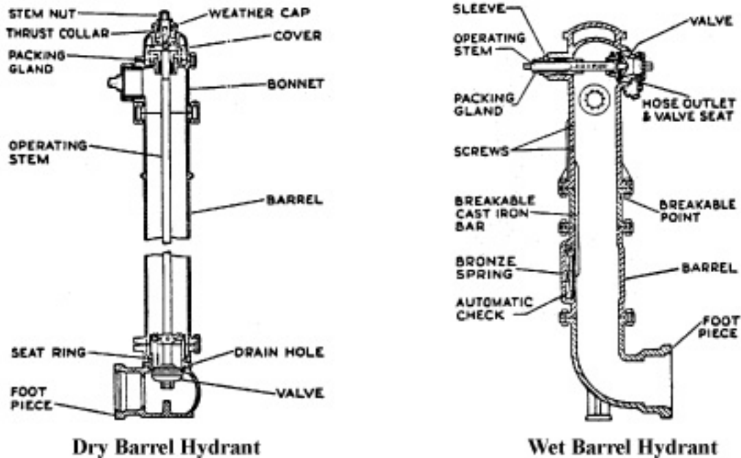
Figure 7.18 - Fire Hydrants
