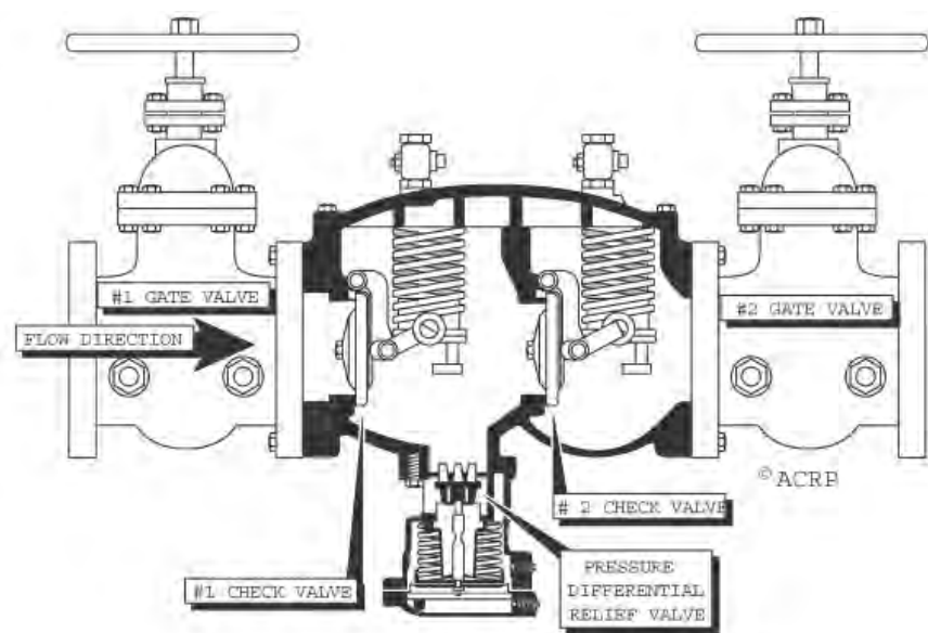
Figure 7.28 - RPZ Device
